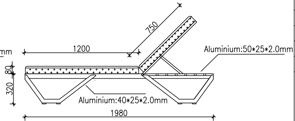
B Side view 侧视图 SCALE 1:15
