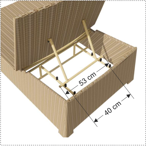
Detail Sandaran
